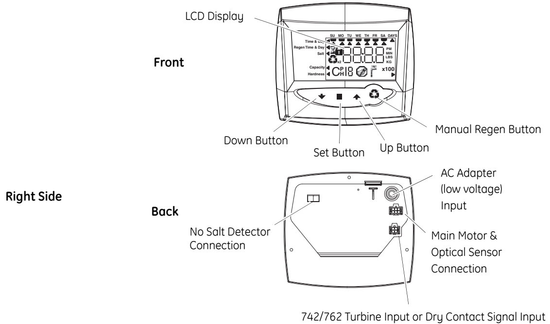
Figure 3 700 Series Controller Identification
